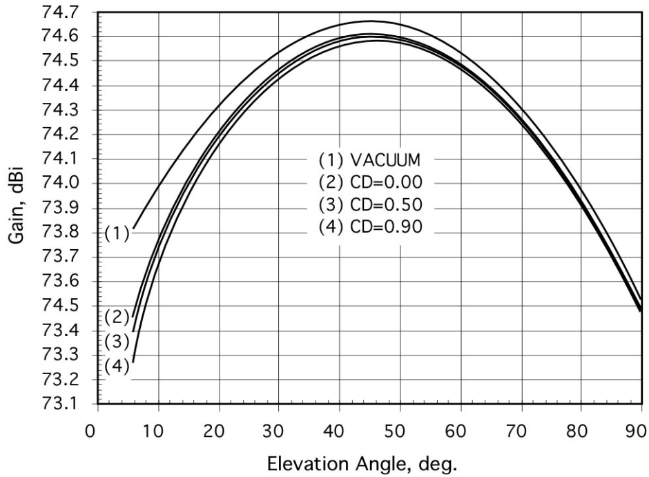
Figure 6. X-Band Receive Gain, DSS 63 Antenna, X-Only Configuration (S/X Dichroic Retracted), at Feedhorn Aperture
