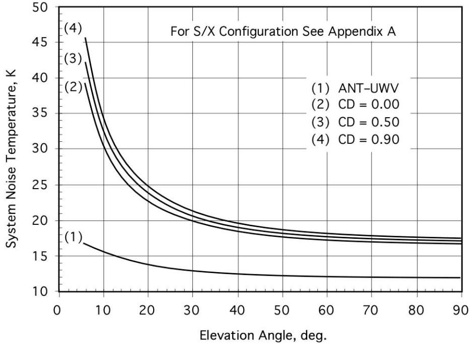
Figure 11. X-Band System Noise Temperature, DSS 14 Antenna, LNA-1 or LNA-2, X-Only Configuration (S/X Dichroic Retracted)
