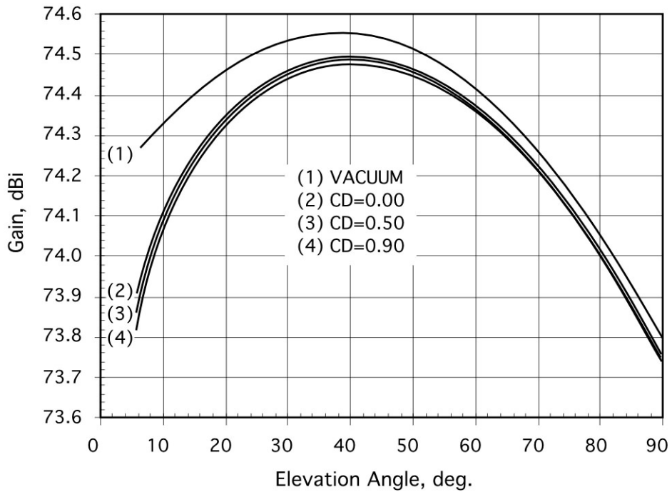
Figure 4. X-Band Receive Gain, DSS 14 Antenna, X-Only Configuration (S/X Dichroic Retracted), at Feedhorn Aperture
