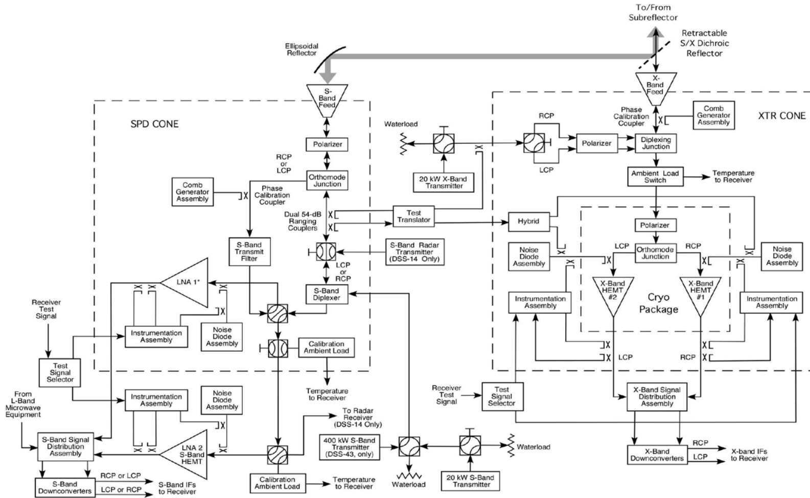
Figure 1. Functional Block Diagram of S-Band and X-Band Microwave and Transmitter Equipment
