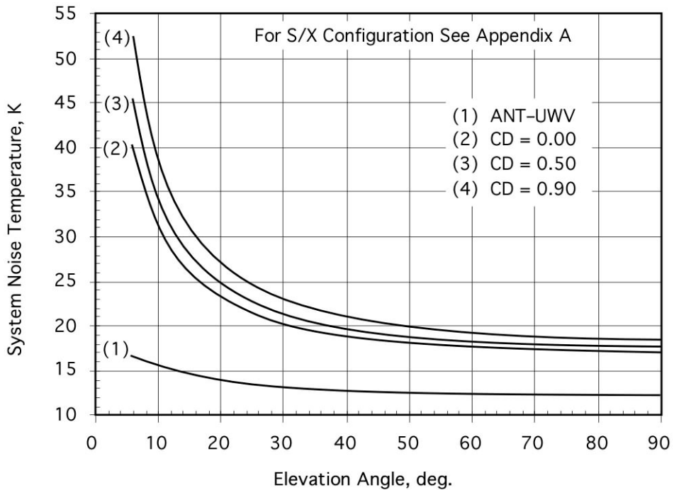
Figure 12. X-Band System Noise Temperature, DSS 43 Antenna, LNA-1 or LNA-2, X-Only Configuration (S/X Dichroic Retracted)
