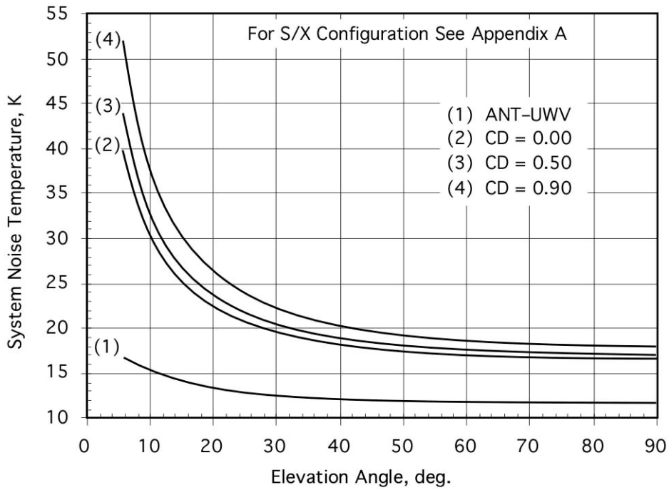
Figure 13. X-Band System Noise Temperature, DSS 63 Antenna, LNA-1 or LNA-2, X-Only Configuration (S/X Dichroic Retracted)
