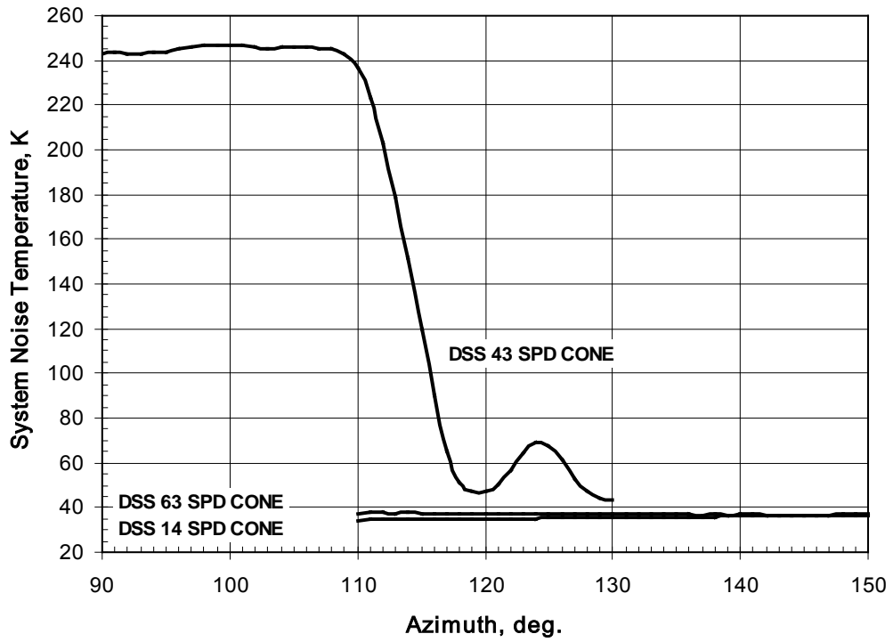
Figure 9. Eastern Horizon S-Band System Noise Temperature at 6° Elevation Angle
