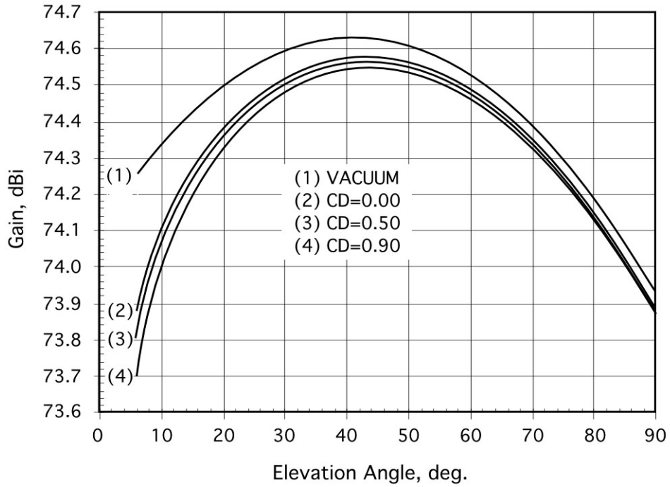
Figure 5. X-Band Receive Gain, DSS 43 Antenna, X-Only Configuration (S/X Dichroic Retracted), at Feedhorn Aperture
