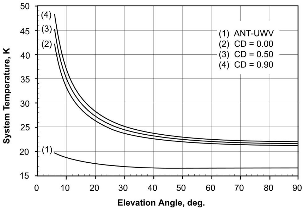
Figure 26. DSS-26 (Goldstone) X-Band RCP System Temperature versus Elevation Angle, X/Ka-Mode, 8420 MHz
