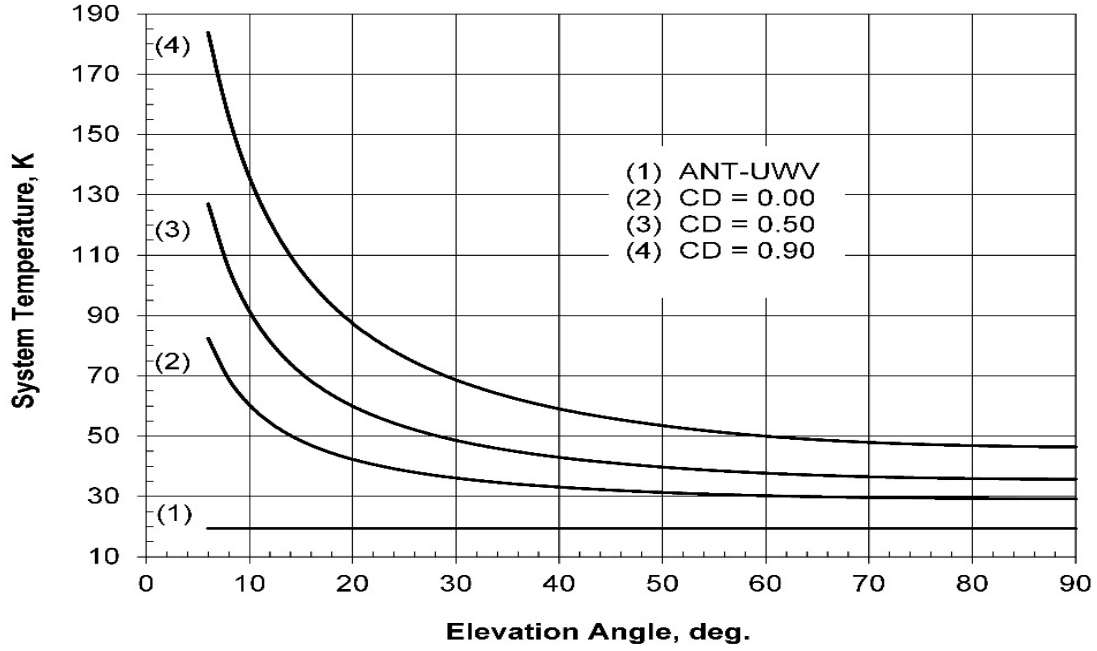
Figure 37. DSS-34 (Canberra) Ka-Band RCP System Temperature versus Elevation Angle, X/Ka-Mode, 32000 MHz
