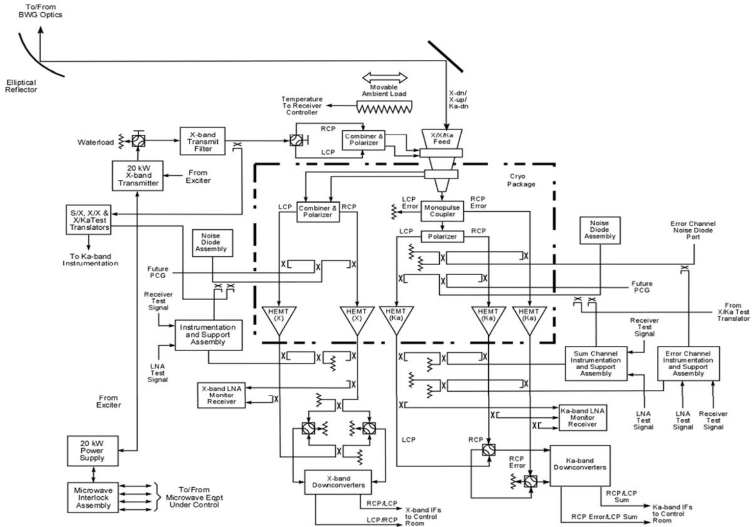
Figure 6. Functional Block Diagram of the DSS-55 Antenna
