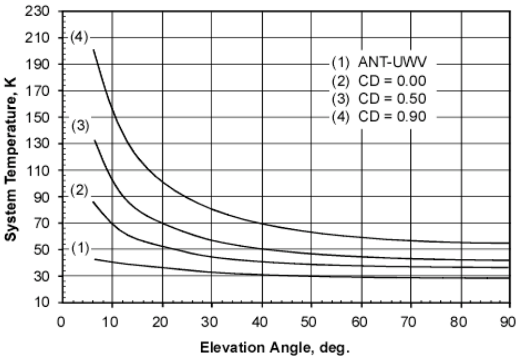
Figure 34. DSS-54 (Madrid) K-Band RCP System Temperature versus Elevation Angle, K-only Mode (S/K Dichroic Retracted), 26000 MHz
