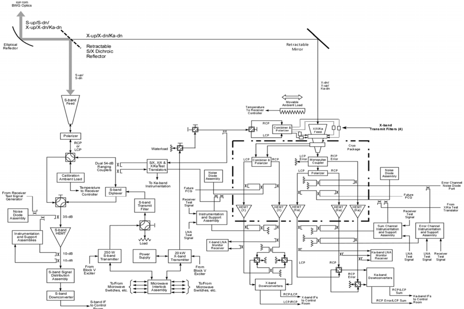
Figure 5. Functional Block Diagram of the DSS-36 Antenna
