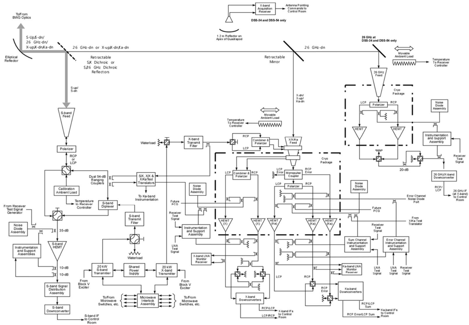
Figure 4. Functional Block Diagram of the DSS-34 and DSS-54 Antennas
