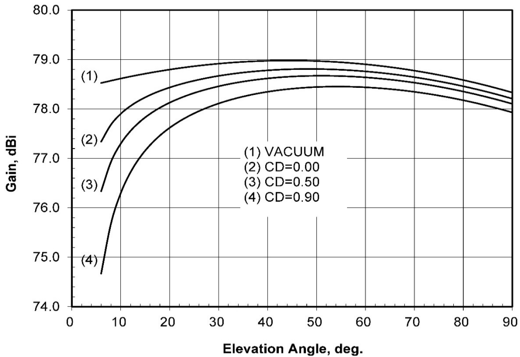
Figure 20. DSS-34 (Canberra) Ka-Band Receive Gain versus Elevation Angle, X/Ka-Mode, 32000 MHz
