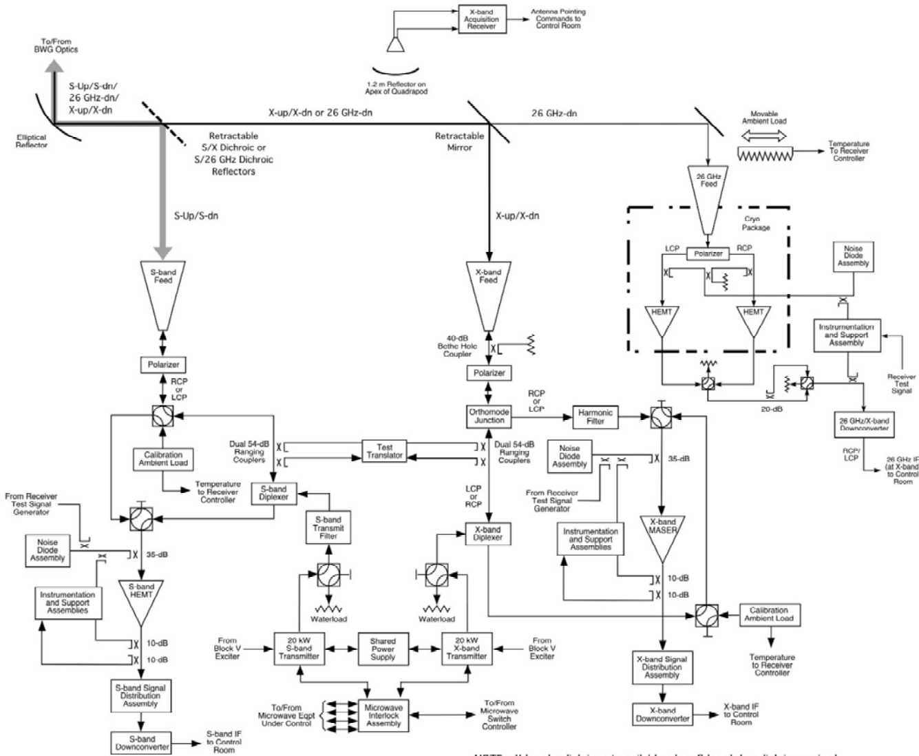
Figure 1. Functional Block Diagram of the DSS-24 Antenna
