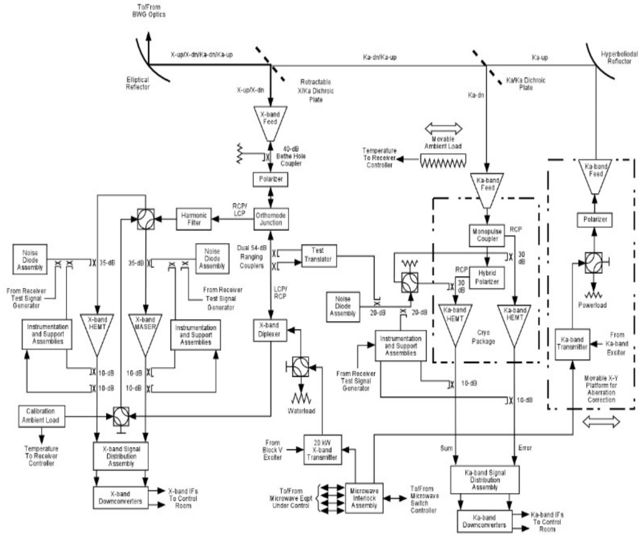
Figure 2. Functional Block Diagram of the DSS-25 Antenna
