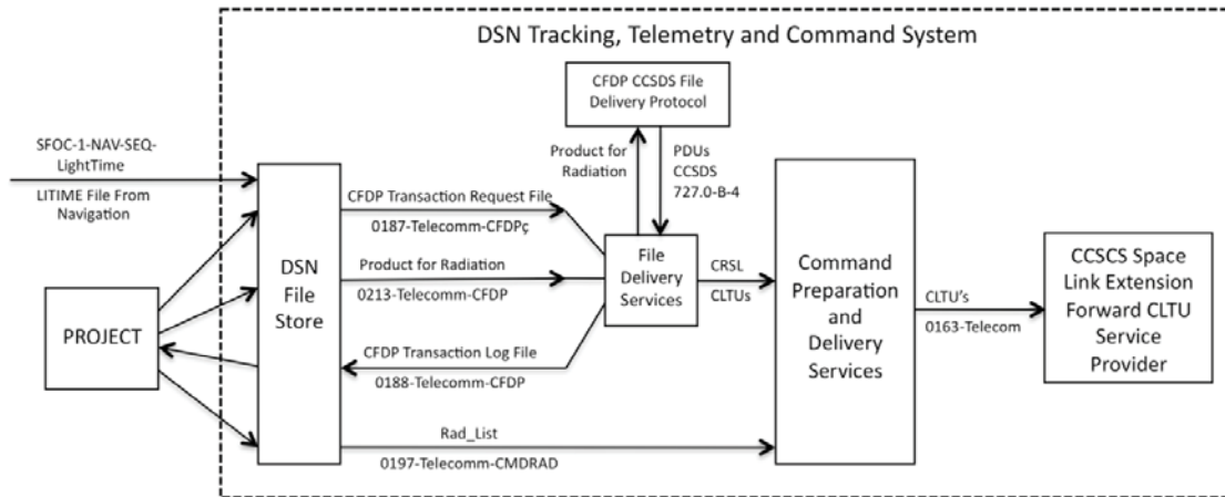
Figure 5. Command Delivery Service Dataflow – (CFDP)
