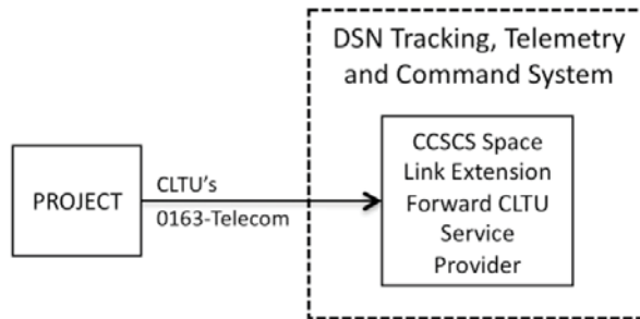
Figure 3. Space Link Extension (SLE) Forward Service Dataflow
