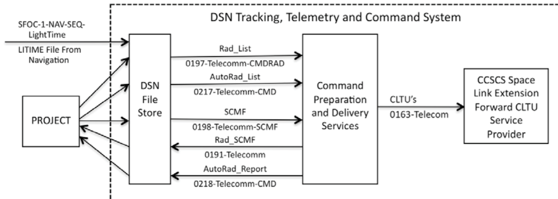
Figure 4. Command Radiation Service Dataflow – File Mode (SCMF)
