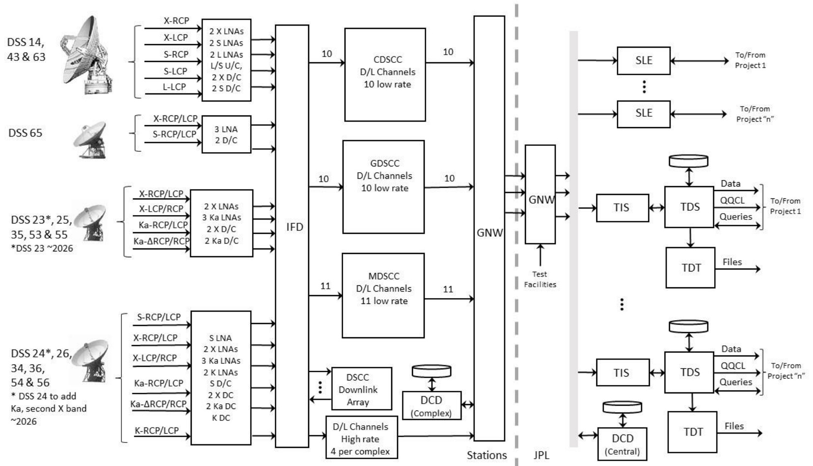
Figure 1. DSN Telemetry Equipment for Spacecraft Support
