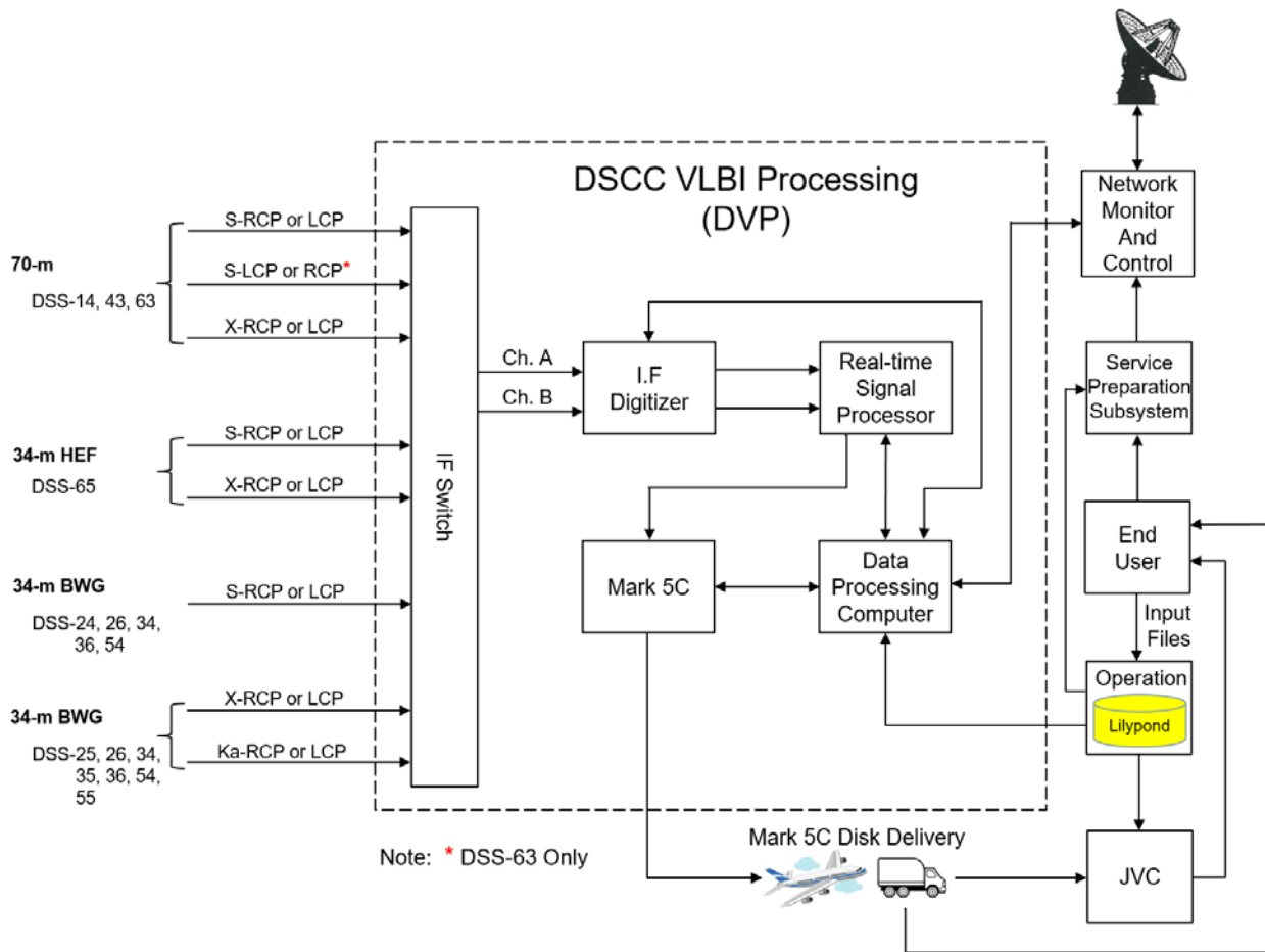
Figure 2. DSN Equipment for Wideband VLBI Support
