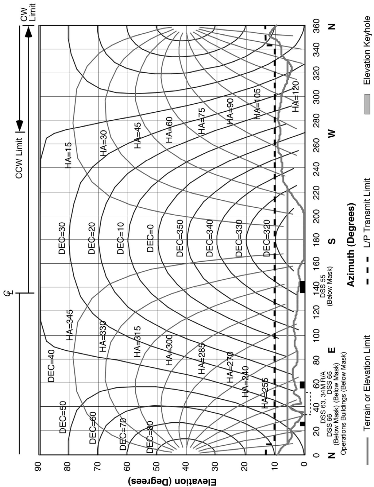
Figure 21. DSS 54 Hour-Angle and Declination Profiles and Horizon Mask
