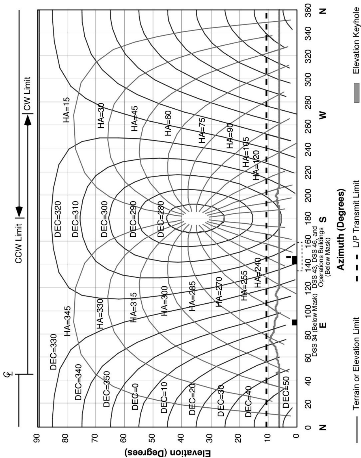
Figure 20. DSS 45 Hour-Angle and Declination Profiles and Horizon Mask
