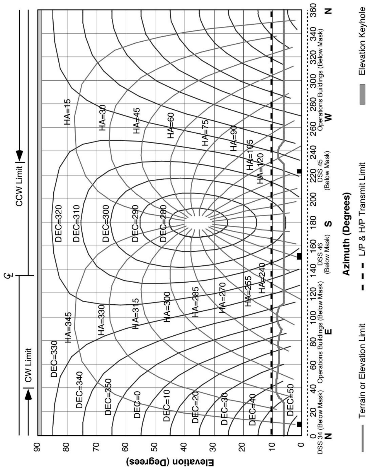
Figure 19. DSS 43 Hour-Angle and Declination Profiles and Horizon Mask
