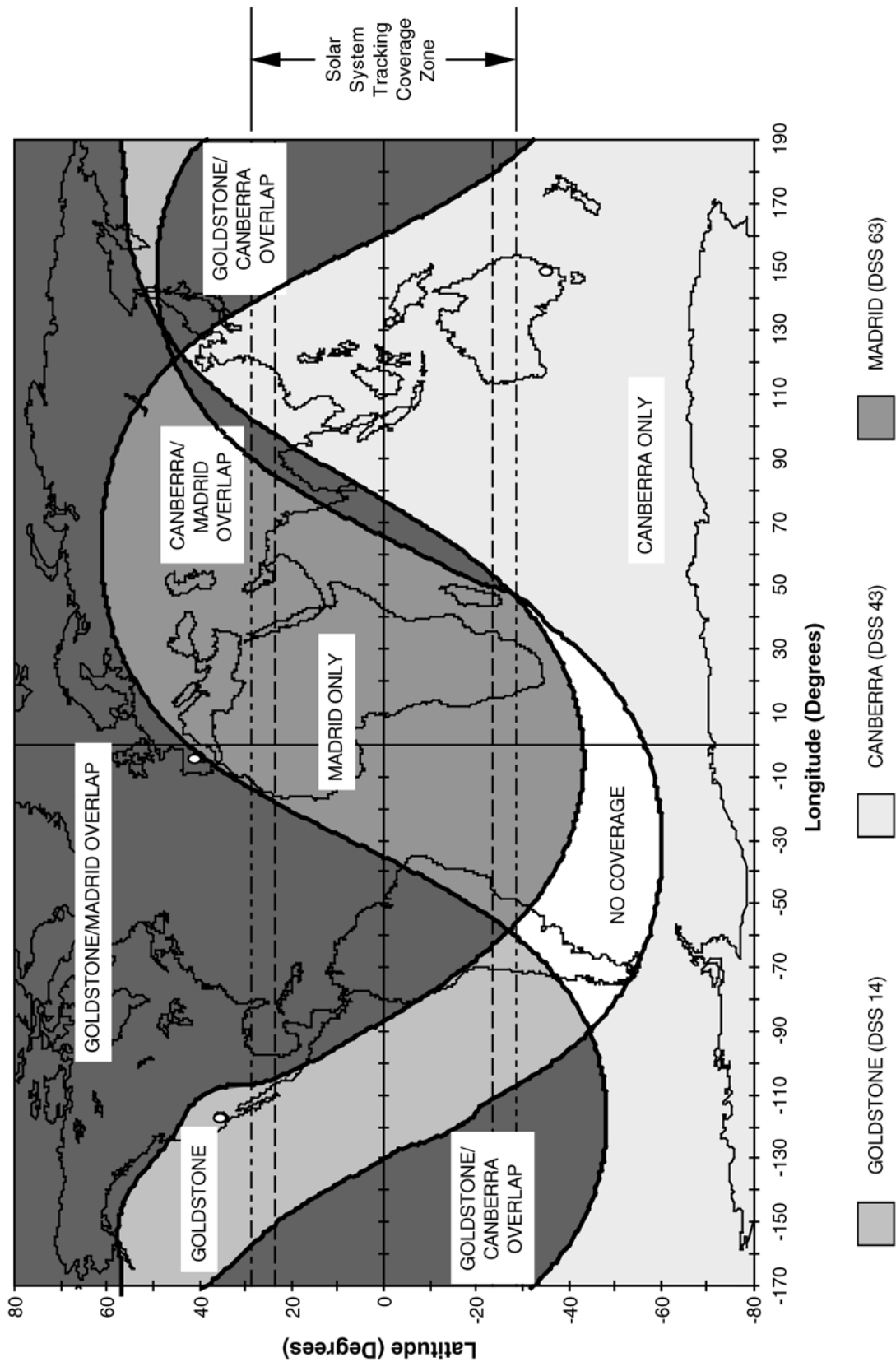
Figure 2. DSN 70-m Subnet Receive Coverage, Planetary Spacecraft
