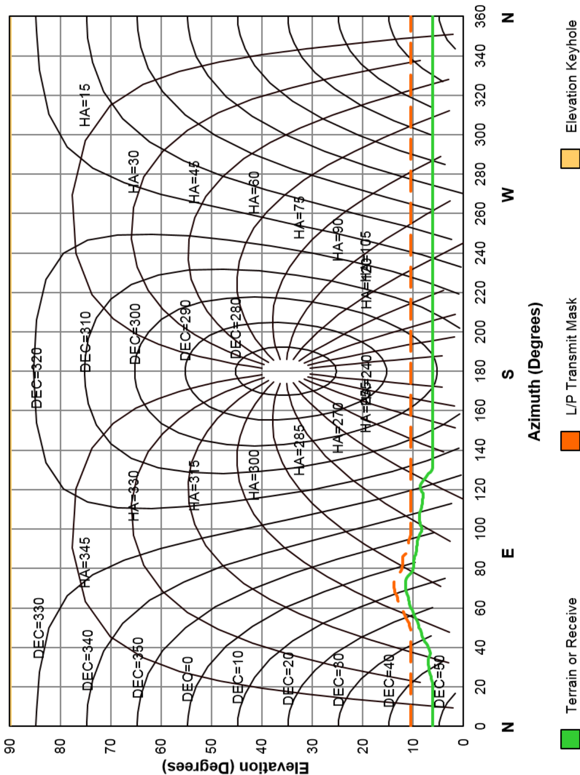
Figure 16. DSS 34 Hour-Angle and Declination Profiles and Horizon Mask
