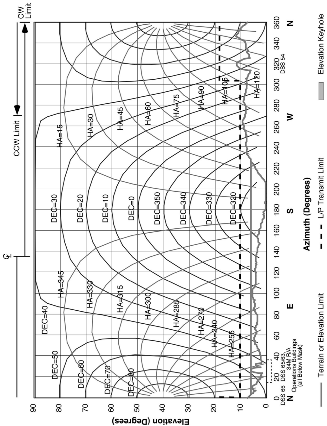
Figure 22. DSS 55 Hour-Angle and Declination Profiles and Horizon Mask
