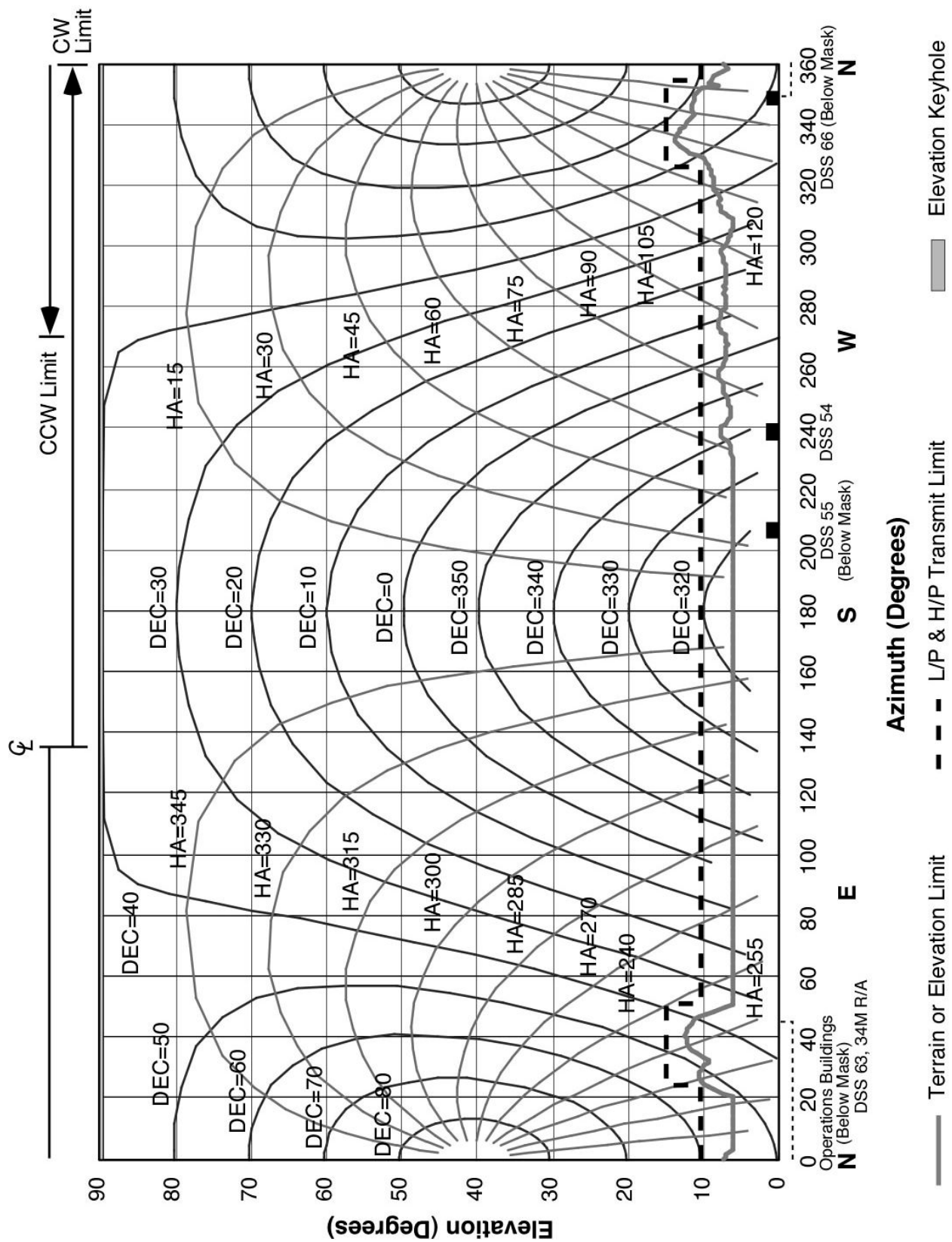
Figure 24. DSS 65 Hour-Angle and Declination Profiles and Horizon Mask
