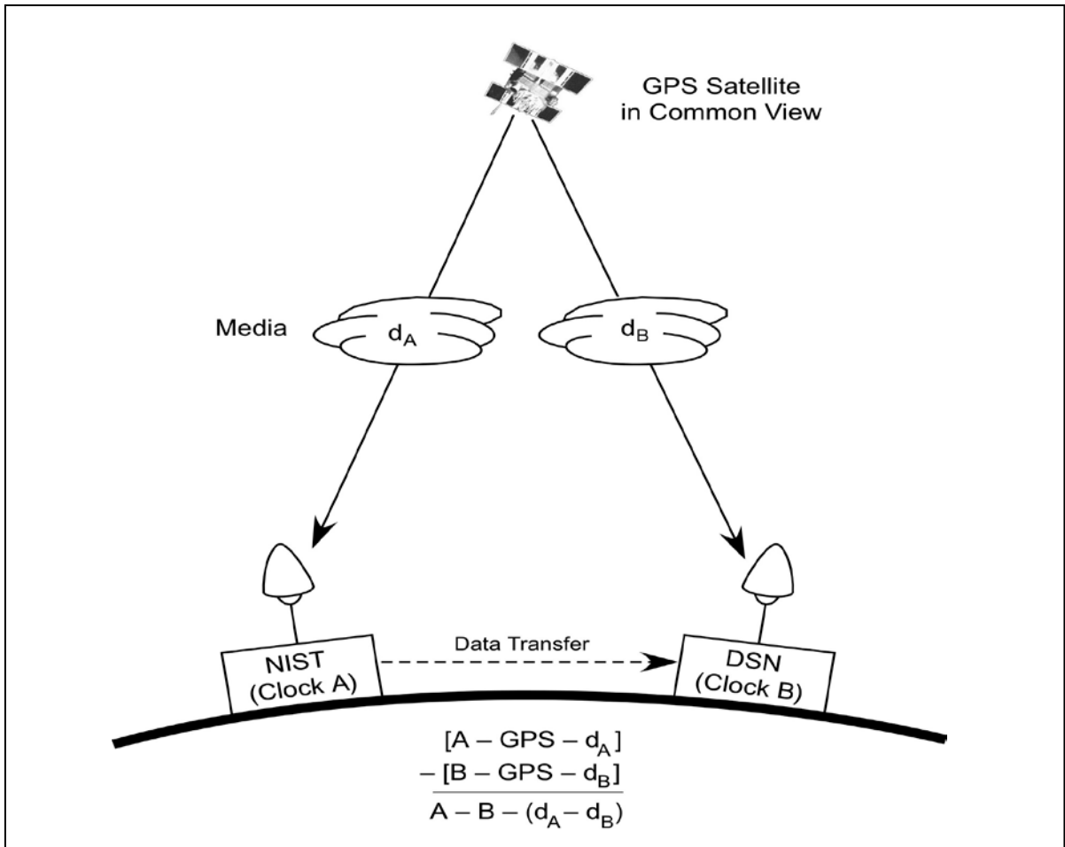
Figure 5. Common-View GPS Time Transfer
